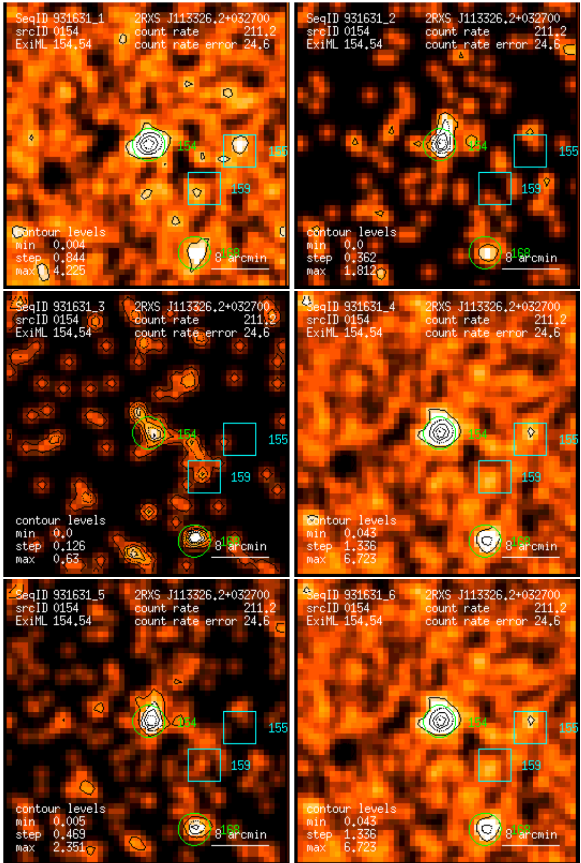
Figure 154: RASS 931631: detection 0154: band rate images, Gaussian filter: (1) PSPC channels 11 – 41, (2) 52 – 90, (3) 91 – 201, (4) 11 – 235, (5) 52 – 201, (6) 11 – 201. Broad band rates in counts/ks. Band rate contour levels in counts/ks/arcmin 2 .
