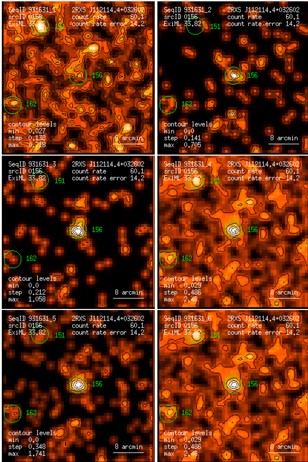
Figure 156: RASS 931631: detection 0156: band rate images, Gaussian filter: (1) PSPC channels 11 – 41, (2) 52 – 90, (3) 91 – 201, (4) 11 – 235, (5) 52 – 201, (6) 11 – 201. Broad band rates in counts/ks. Band rate contour levels in counts/ks/arcmin 2 .
