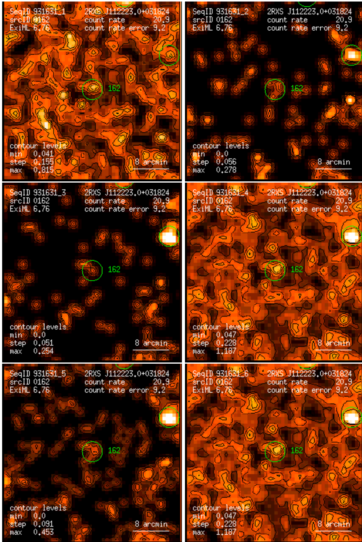
Figure 162: RASS 931631: detection 0162: band rate images, Gaussian filter: (1) PSPC channels 11 – 41, (2) 52 – 90, (3) 91 – 201, (4) 11 – 235, (5) 52 – 201, (6) 11 – 201. Broad band rates in counts/ks. Band rate contour levels in counts/ks/arcmin 2 .
