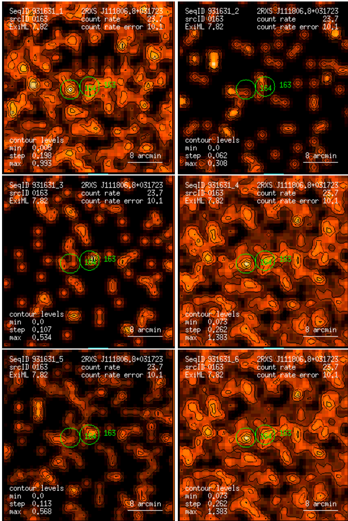
Figure 163: RASS 931631: detection 0163: band rate images, Gaussian filter: (1) PSPC channels 11 – 41, (2) 52 – 90, (3) 91 – 201, (4) 11 – 235, (5) 52 – 201, (6) 11 – 201. Broad band rates in counts/ks. Band rate contour levels in counts/ks/arcmin 2 .
