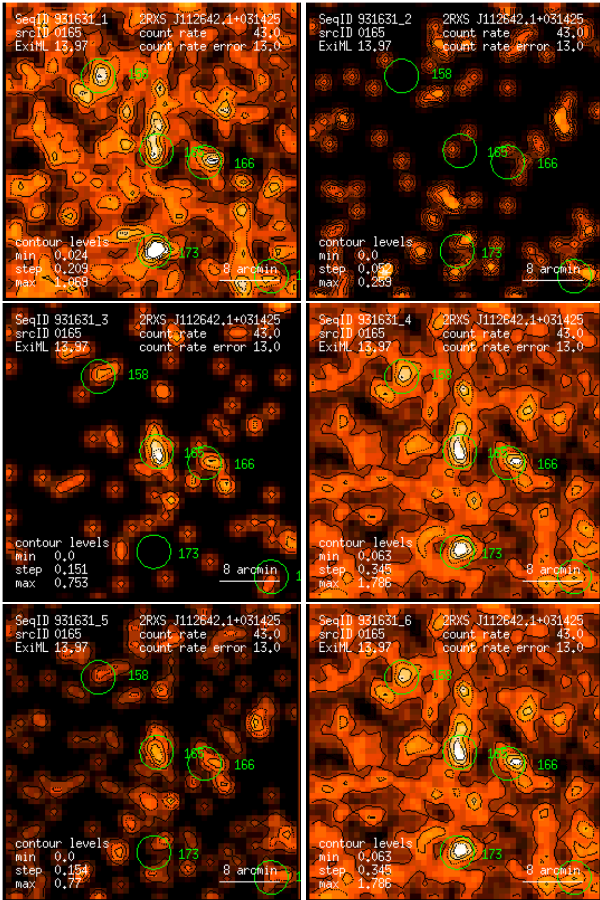
Figure 165: RASS 931631: detection 0165: band rate images, Gaussian filter: (1) PSPC channels 11 – 41, (2) 52 – 90, (3) 91 – 201, (4) 11 – 235, (5) 52 – 201, (6) 11 – 201. Broad band rates in counts/ks. Band rate contour levels in counts/ks/arcmin 2 .
