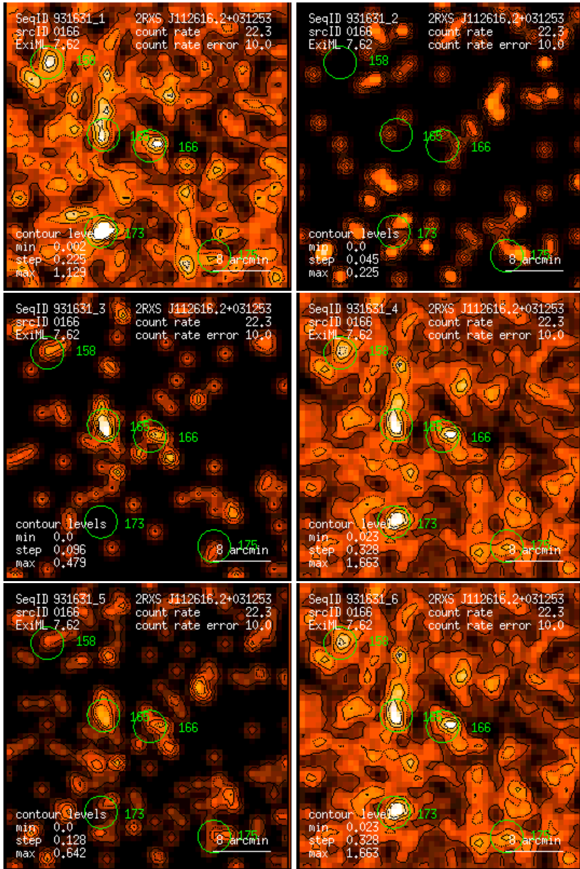
Figure 166: RASS 931631: detection 0166: band rate images, Gaussian filter: (1) PSPC channels 11 – 41, (2) 52 – 90, (3) 91 – 201, (4) 11 – 235, (5) 52 – 201, (6) 11 – 201. Broad band rates in counts/ks. Band rate contour levels in counts/ks/arcmin 2 .
