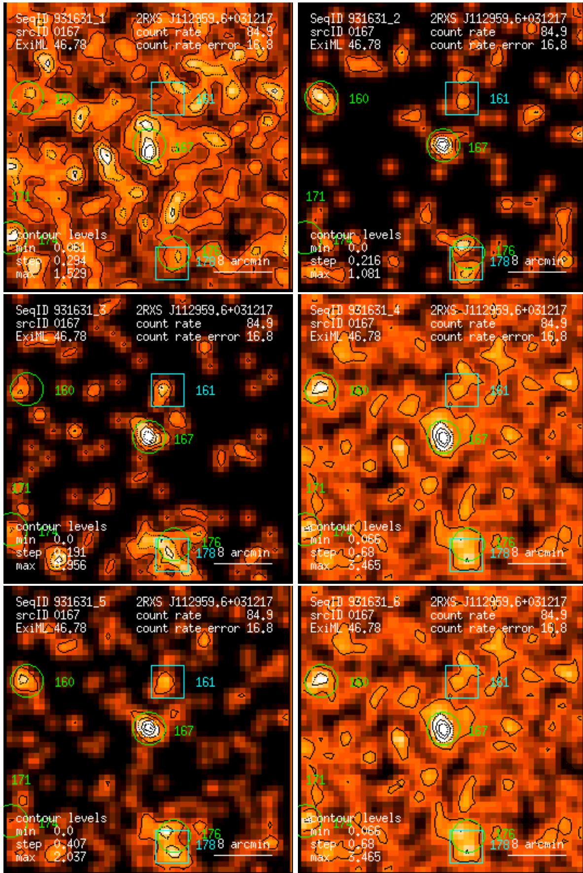
Figure 167: RASS 931631: detection 0167: band rate images, Gaussian filter: (1) PSPC channels 11 – 41, (2) 52 – 90, (3) 91 – 201, (4) 11 – 235, (5) 52 – 201, (6) 11 – 201. Broad band rates in counts/ks. Band rate contour levels in counts/ks/arcmin 2 .
