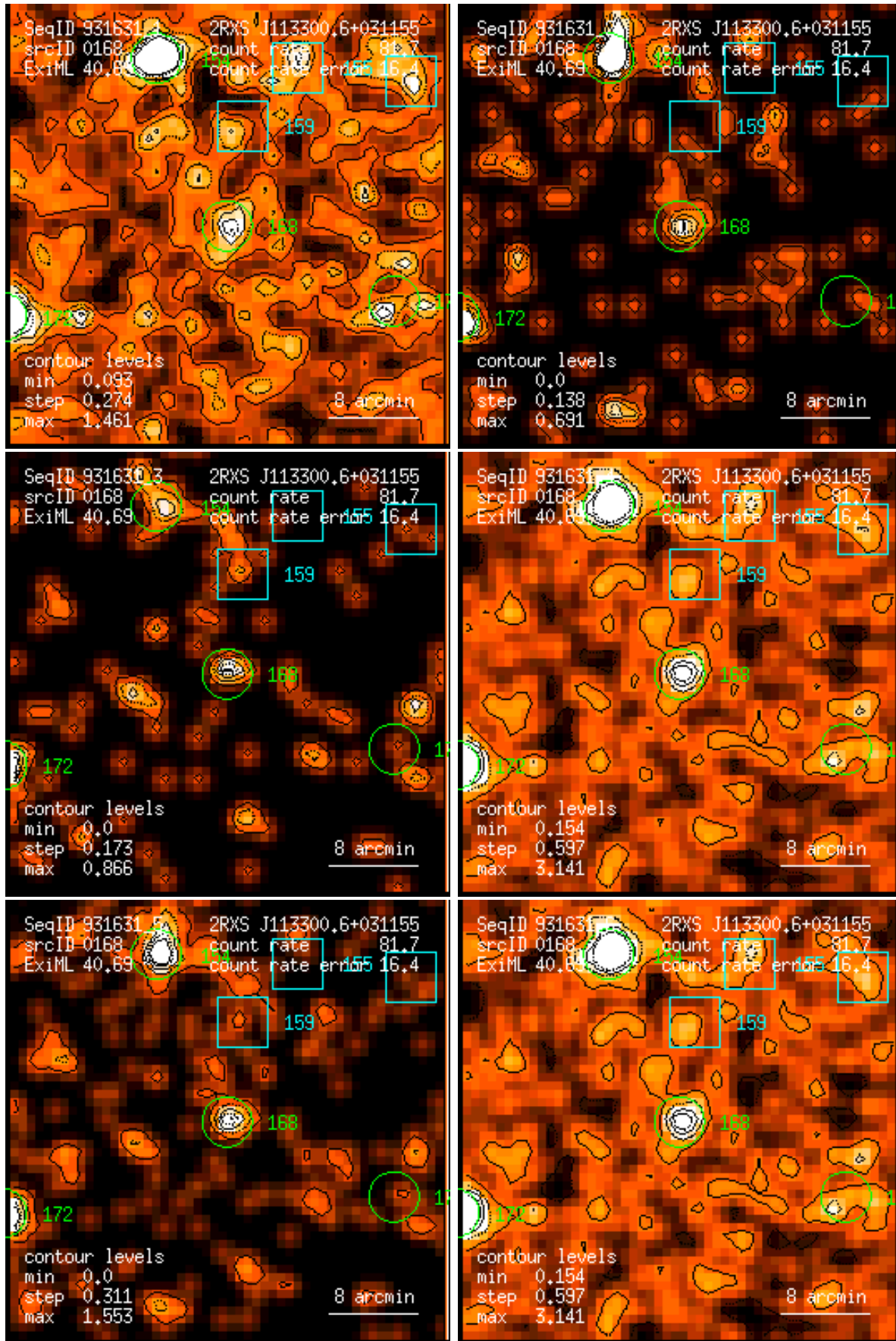
Figure 168: RASS 931631: detection 0168: band rate images, Gaussian filter: (1) PSPC channels 11 – 41, (2) 52 – 90, (3) 91 – 201, (4) 11 – 235, (5) 52 – 201, (6) 11 – 201. Broad band rates in counts/ks. Band rate contour levels in counts/ks/arcmin 2 .
