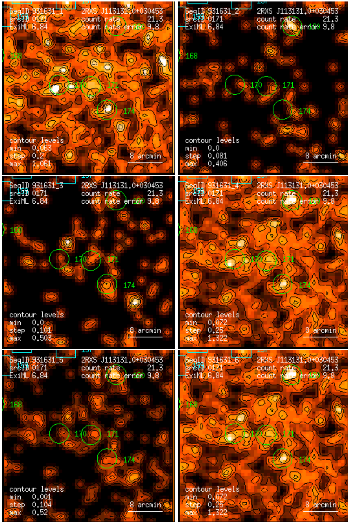
Figure 171: RASS 931631: detection 0171: band rate images, Gaussian filter: (1) PSPC channels 11 – 41, (2) 52 – 90, (3) 91 – 201, (4) 11 – 235, (5) 52 – 201, (6) 11 – 201. Broad band rates in counts/ks. Band rate contour levels in counts/ks/arcmin 2 .
