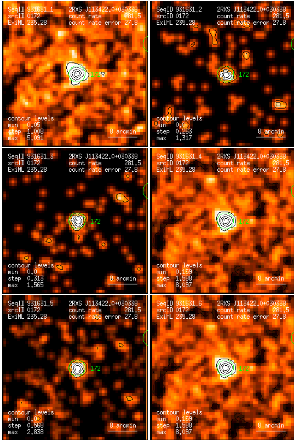
Figure 172: RASS 931631: detection 0172: band rate images, Gaussian filter: (1) PSPC channels 11 – 41, (2) 52 – 90, (3) 91 – 201, (4) 11 – 235, (5) 52 – 201, (6) 11 – 201. Broad band rates in counts/ks. Band rate contour levels in counts/ks/arcmin 2 .
