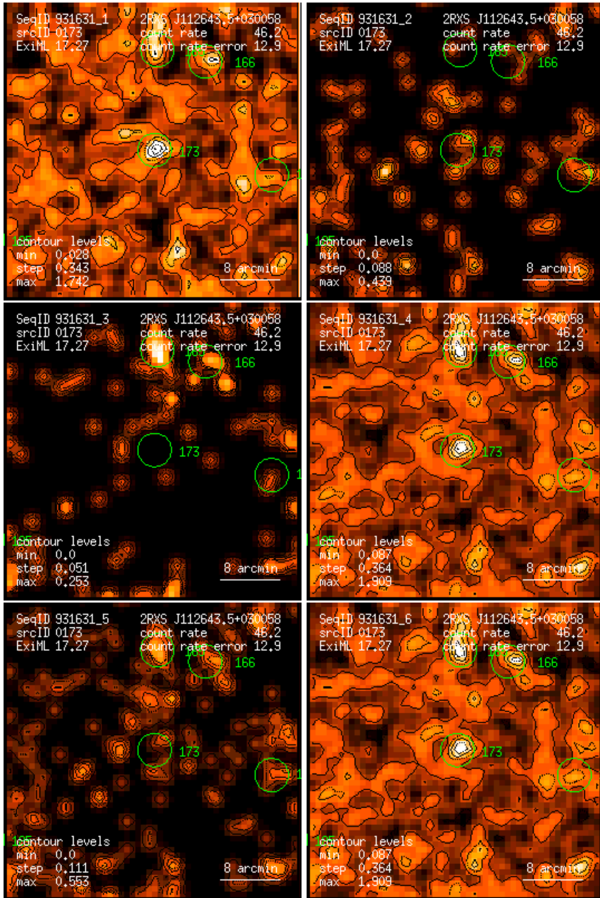
Figure 173: RASS 931631: detection 0173: band rate images, Gaussian filter: (1) PSPC channels 11 – 41, (2) 52 – 90, (3) 91 – 201, (4) 11 – 235, (5) 52 – 201, (6) 11 – 201. Broad band rates in counts/ks. Band rate contour levels in counts/ks/arcmin 2 .
