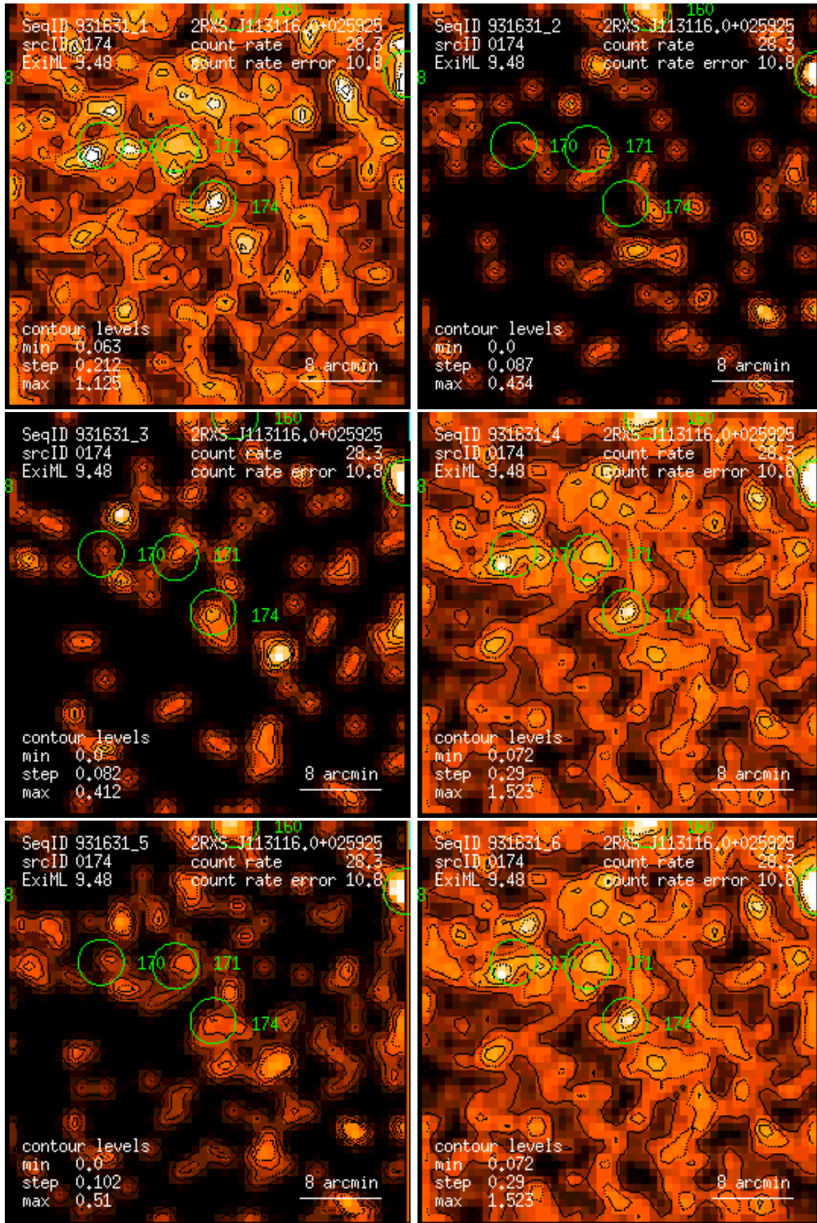
Figure 174: RASS 931631: detection 0174: band rate images, Gaussian filter: (1) PSPC channels 11 – 41, (2) 52 – 90, (3) 91 – 201, (4) 11 – 235, (5) 52 – 201, (6) 11 – 201. Broad band rates in counts/ks. Band rate contour levels in counts/ks/arcmin 2 .
