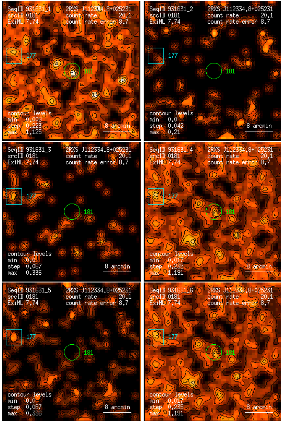
Figure 181: RASS 931631: detection 0181: band rate images, Gaussian filter: (1) PSPC channels 11 – 41, (2) 52 – 90, (3) 91 – 201, (4) 11 – 235, (5) 52 – 201, (6) 11 – 201. Broad band rates in counts/ks. Band rate contour levels in counts/ks/arcmin 2 .
