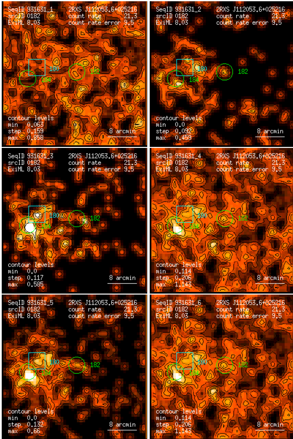
Figure 182: RASS 931631: detection 0182: band rate images, Gaussian filter: (1) PSPC channels 11 – 41, (2) 52 – 90, (3) 91 – 201, (4) 11 – 235, (5) 52 – 201, (6) 11 – 201. Broad band rates in counts/ks. Band rate contour levels in counts/ks/arcmin 2 .
