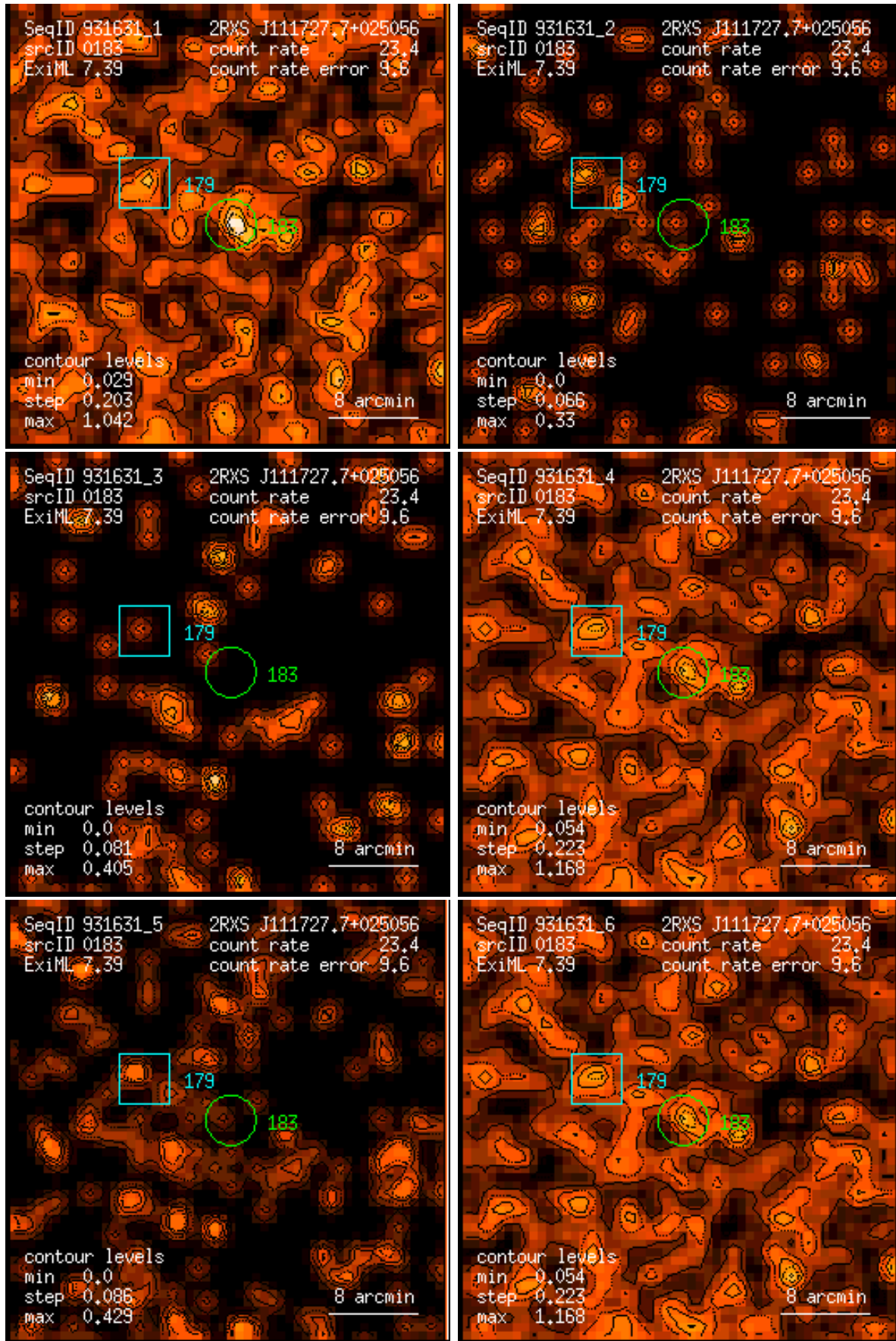
Figure 183: RASS 931631: detection 0183: band rate images, Gaussian filter: (1) PSPC channels 11 – 41, (2) 52 – 90, (3) 91 – 201, (4) 11 – 235, (5) 52 – 201, (6) 11 – 201. Broad band rates in counts/ks. Band rate contour levels in counts/ks/arcmin 2 .
