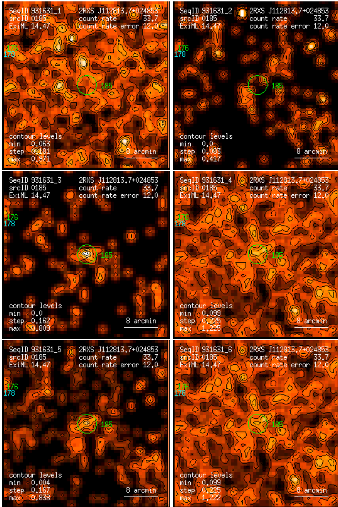
Figure 185: RASS 931631: detection 0185: band rate images, Gaussian filter: (1) PSPC channels 11 – 41, (2) 52 – 90, (3) 91 – 201, (4) 11 – 235, (5) 52 – 201, (6) 11 – 201. Broad band rates in counts/ks. Band rate contour levels in counts/ks/arcmin 2 .
