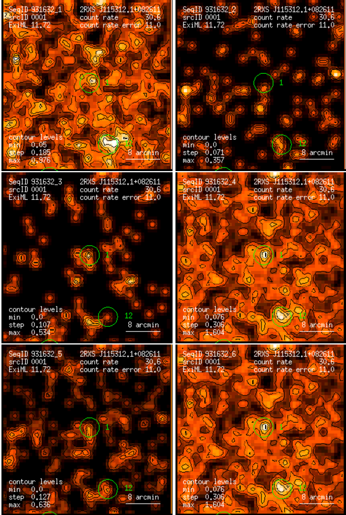
Figure 1: RASS 931632: detection 0001: band rate images, Gaussian filter: (1) PSPC channels 11 – 41, (2) 52 – 90, (3) 91 – 201, (4) 11 – 235, (5) 52 – 201, (6) 11 – 201. Broad band rates in counts/ks. Band rate contour levels in counts/ks/arcmin 2 .
