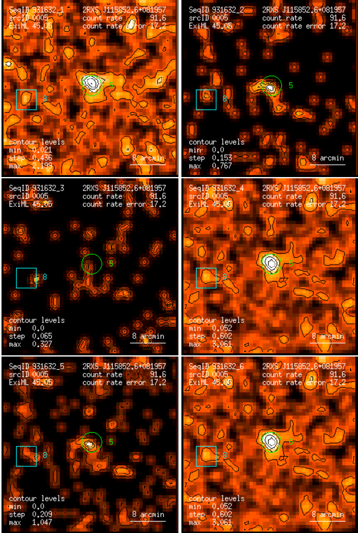
Figure 5: RASS 931632: detection 0005: band rate images, Gaussian filter: (1) PSPC channels 11 – 41, (2) 52 – 90, (3) 91 – 201, (4) 11 – 235, (5) 52 – 201, (6) 11 – 201. Broad band rates in counts/ks. Band rate contour levels in counts/ks/arcmin 2 .
