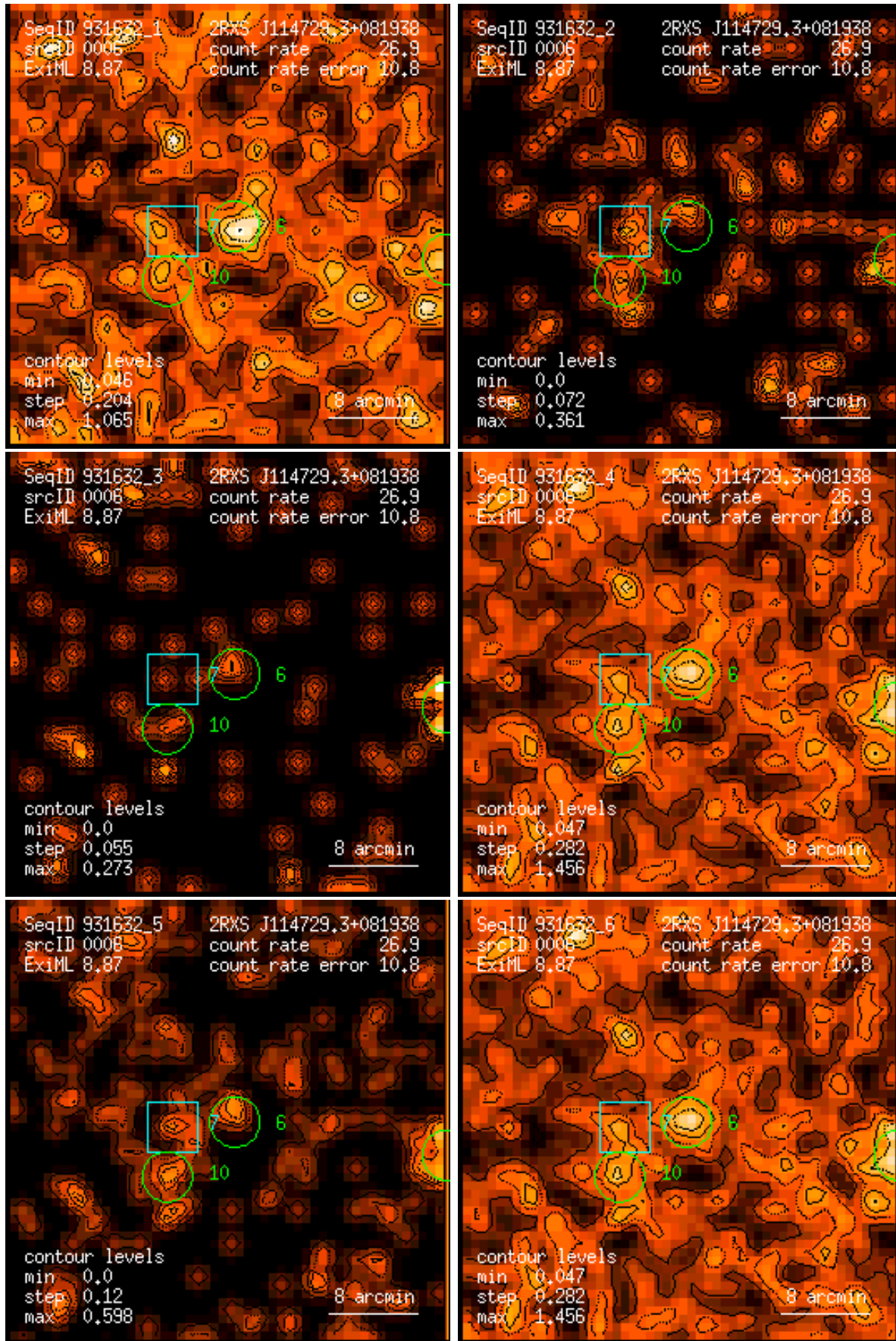
Figure 6: RASS 931632: detection 0006: band rate images, Gaussian filter: (1) PSPC channels 11 – 41, (2) 52 – 90, (3) 91 – 201, (4) 11 – 235, (5) 52 – 201, (6) 11 – 201. Broad band rates in counts/ks. Band rate contour levels in counts/ks/arcmin 2 .
