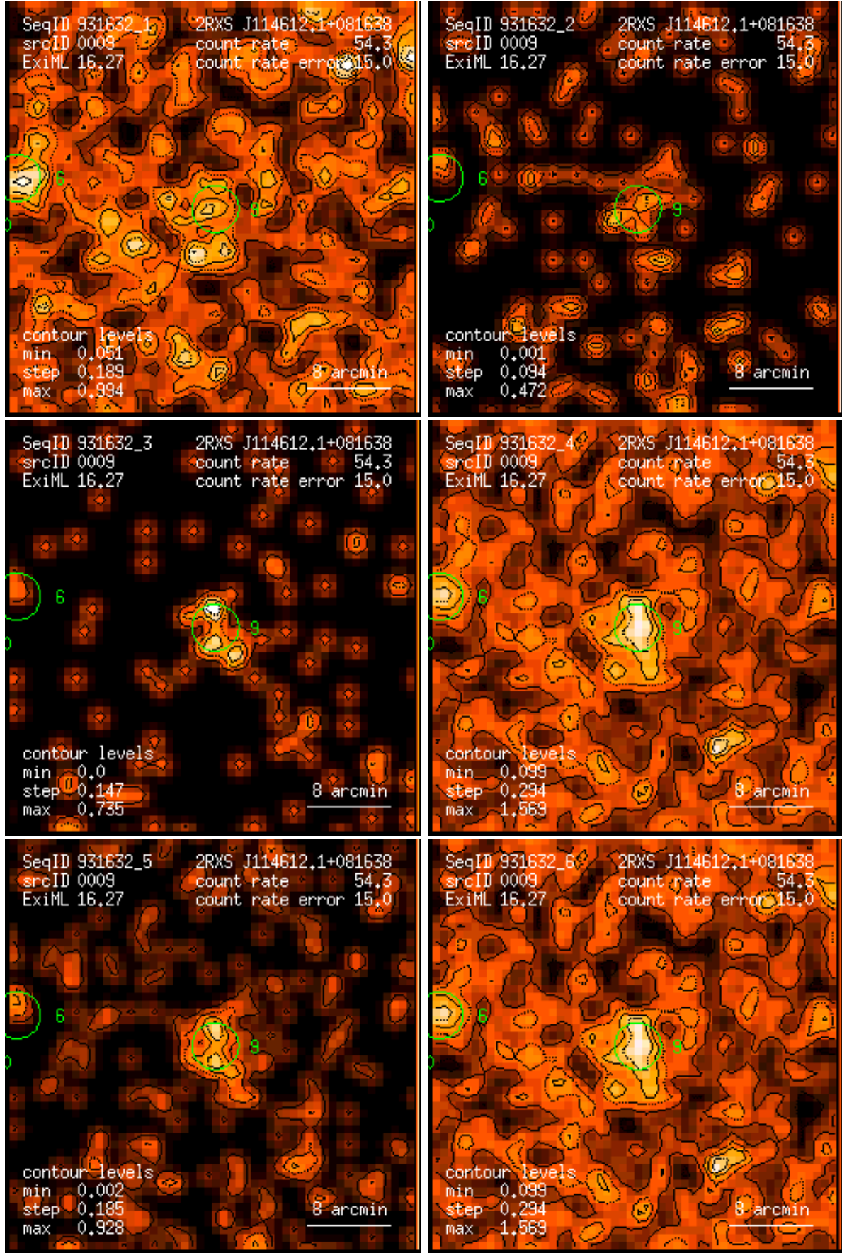
Figure 9: RASS 931632: detection 0009: band rate images, Gaussian filter: (1) PSPC channels 11 – 41, (2) 52 – 90, (3) 91 – 201, (4) 11 – 235, (5) 52 – 201, (6) 11 – 201. Broad band rates in counts/ks. Band rate contour levels in counts/ks/arcmin 2 .
