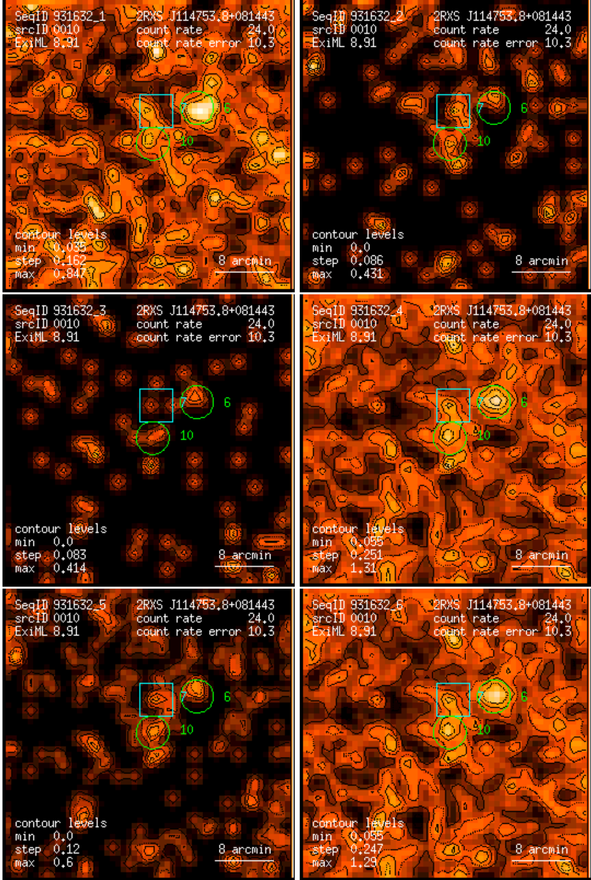
Figure 10: RASS 931632: detection 0010: band rate images, Gaussian filter: (1) PSPC channels 11 – 41, (2) 52 – 90, (3) 91 – 201, (4) 11 – 235, (5) 52 – 201, (6) 11 – 201. Broad band rates in counts/ks. Band rate contour levels in counts/ks/arcmin 2 .
