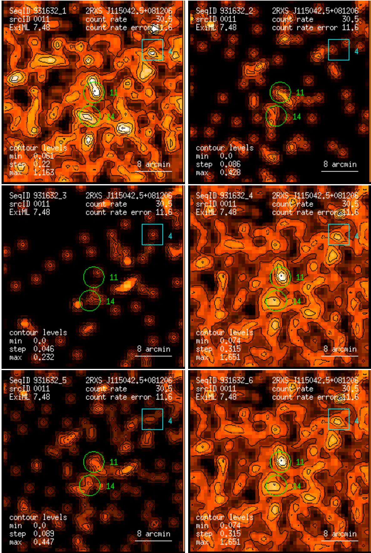
Figure 11: RASS 931632: detection 0011: band rate images, Gaussian filter: (1) PSPC channels 11 – 41, (2) 52 – 90, (3) 91 – 201, (4) 11 – 235, (5) 52 – 201, (6) 11 – 201. Broad band rates in counts/ks. Band rate contour levels in counts/ks/arcmin 2 .
