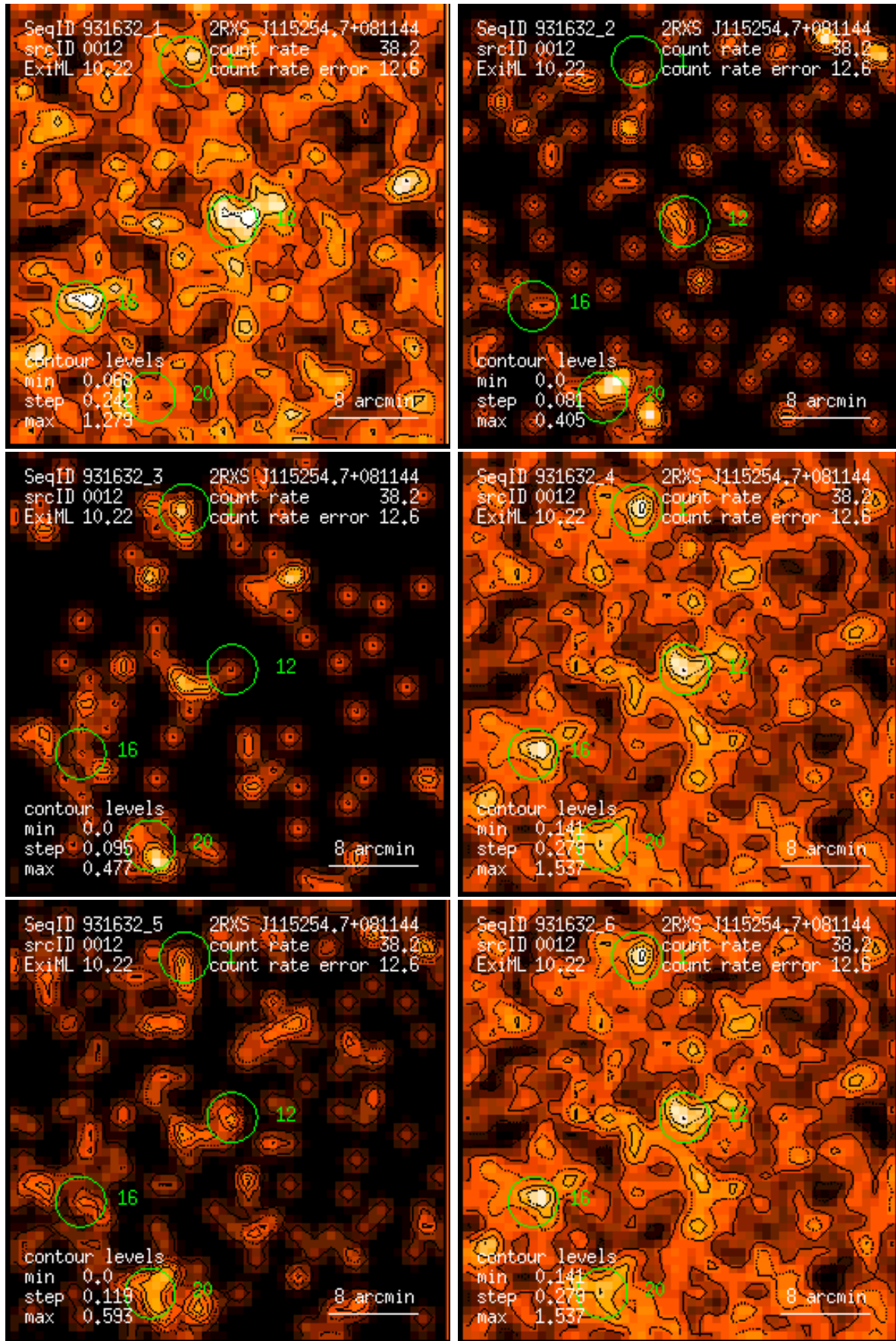
Figure 12: RASS 931632: detection 0012: band rate images, Gaussian filter: (1) PSPC channels 11 – 41, (2) 52 – 90, (3) 91 – 201, (4) 11 – 235, (5) 52 – 201, (6) 11 – 201. Broad band rates in counts/ks. Band rate contour levels in counts/ks/arcmin 2 .
