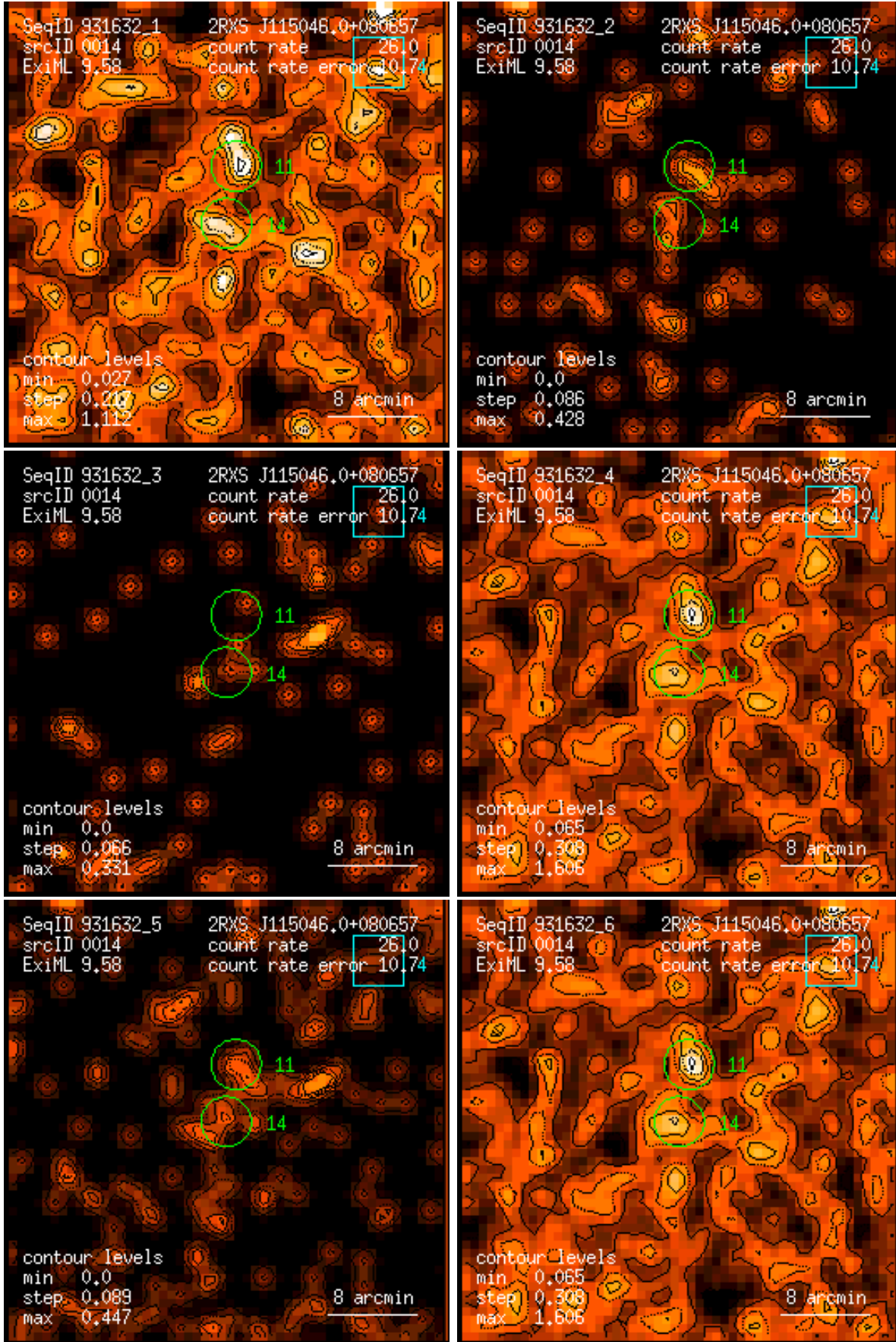
Figure 14: RASS 931632: detection 0014: band rate images, Gaussian filter: (1) PSPC channels 11 – 41, (2) 52 – 90, (3) 91 – 201, (4) 11 – 235, (5) 52 – 201, (6) 11 – 201. Broad band rates in counts/ks. Band rate contour levels in counts/ks/arcmin 2 .
