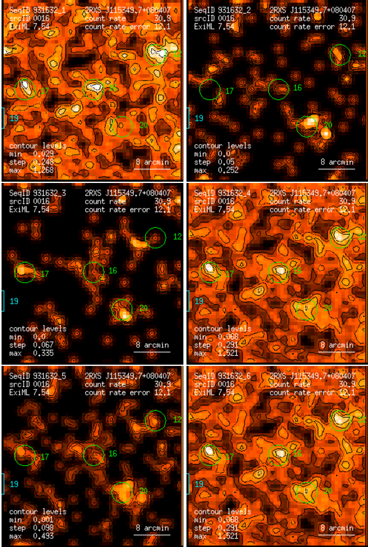
Figure 16: RASS 931632: detection 0016: band rate images, Gaussian filter: (1) PSPC channels 11 – 41, (2) 52 – 90, (3) 91 – 201, (4) 11 – 235, (5) 52 – 201, (6) 11 – 201. Broad band rates in counts/ks. Band rate contour levels in counts/ks/arcmin 2 .
