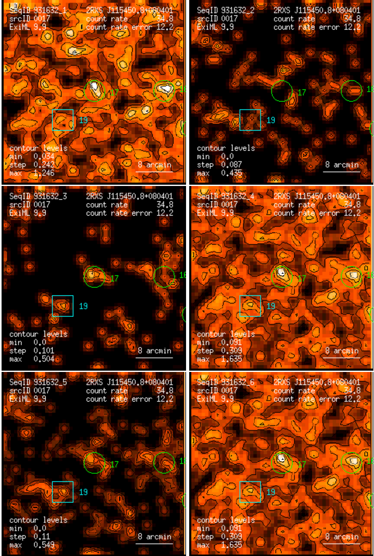
Figure 17: RASS 931632: detection 0017: band rate images, Gaussian filter: (1) PSPC channels 11 – 41, (2) 52 – 90, (3) 91 – 201, (4) 11 – 235, (5) 52 – 201, (6) 11 – 201. Broad band rates in counts/ks. Band rate contour levels in counts/ks/arcmin 2 .
