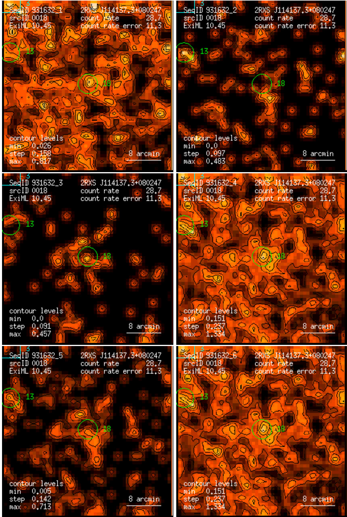
Figure 18: RASS 931632: detection 0018: band rate images, Gaussian filter: (1) PSPC channels 11 – 41, (2) 52 – 90, (3) 91 – 201, (4) 11 – 235, (5) 52 – 201, (6) 11 – 201. Broad band rates in counts/ks. Band rate contour levels in counts/ks/arcmin 2 .
