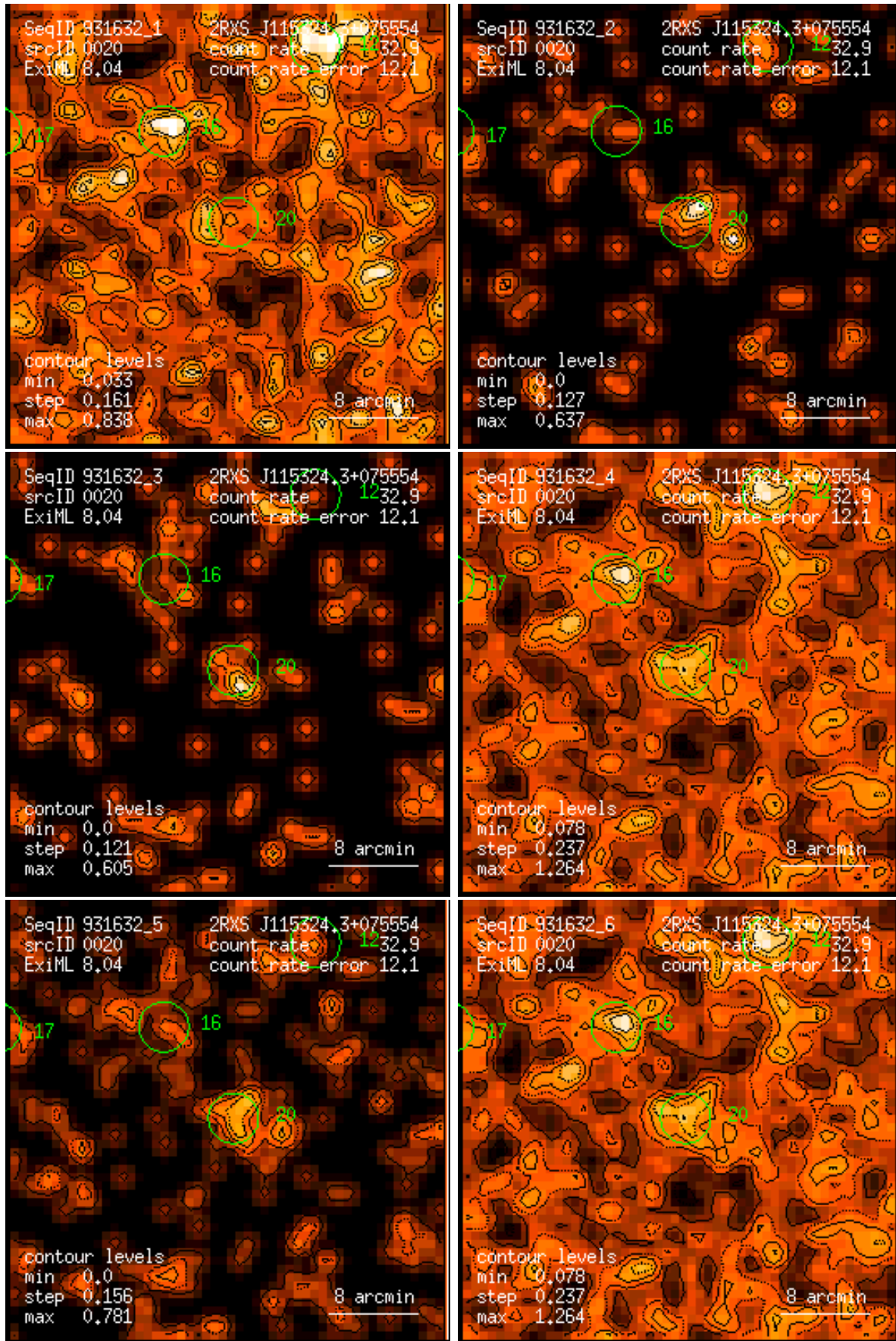
Figure 20: RASS 931632: detection 0020: band rate images, Gaussian filter: (1) PSPC channels 11 – 41, (2) 52 – 90, (3) 91 – 201, (4) 11 – 235, (5) 52 – 201, (6) 11 – 201. Broad band rates in counts/ks. Band rate contour levels in counts/ks/arcmin 2 .
