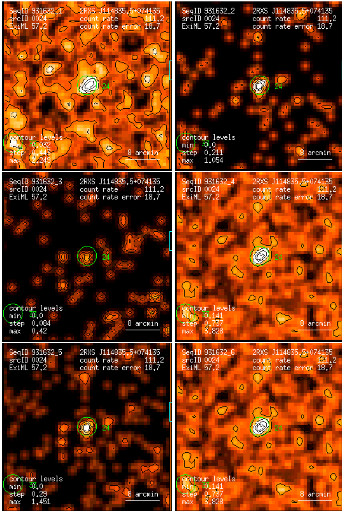
Figure 24: RASS 931632: detection 0024: band rate images, Gaussian filter: (1) PSPC channels 11 – 41, (2) 52 – 90, (3) 91 – 201, (4) 11 – 235, (5) 52 – 201, (6) 11 – 201. Broad band rates in counts/ks. Band rate contour levels in counts/ks/arcmin 2 .
