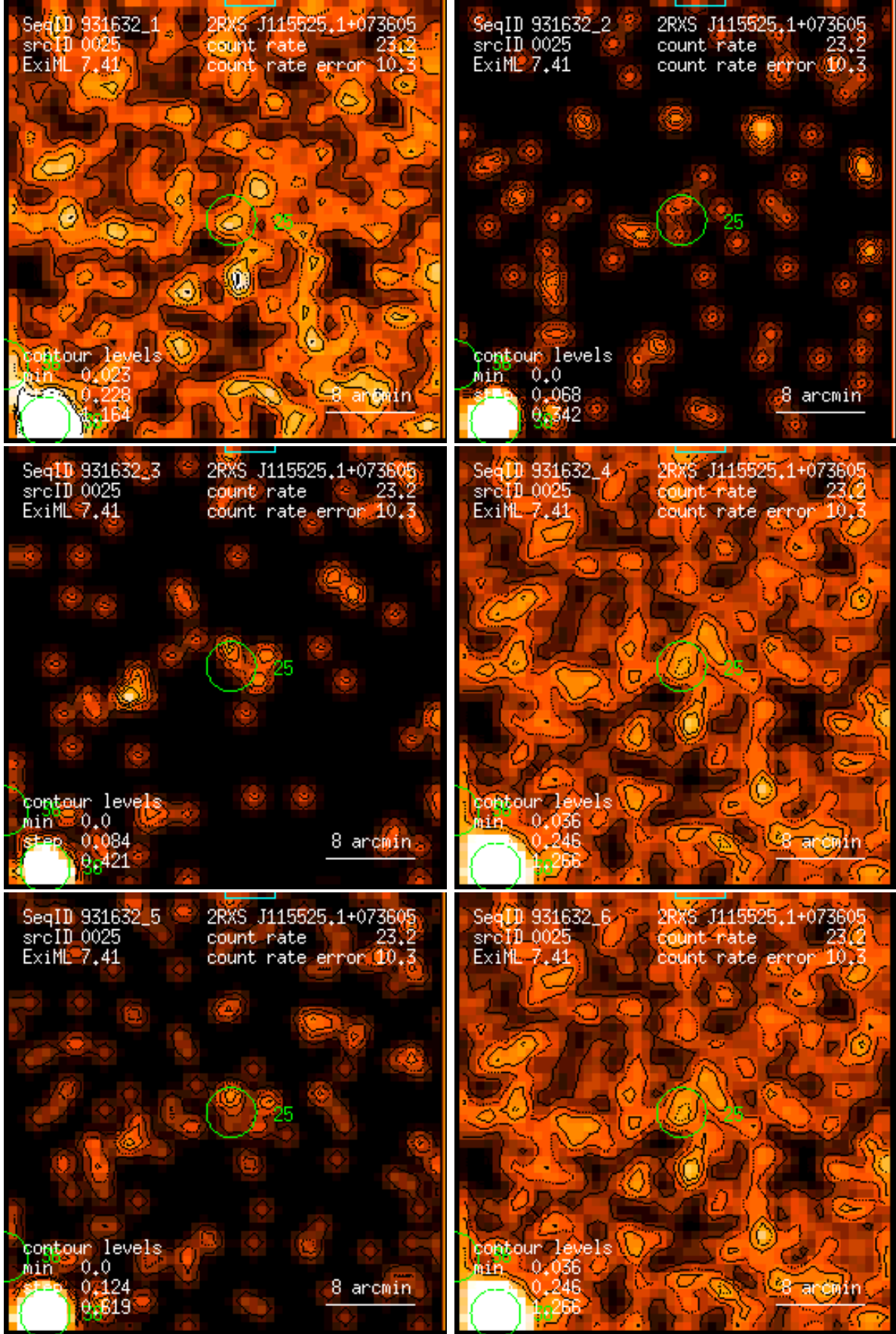
Figure 25: RASS 931632: detection 0025: band rate images, Gaussian filter: (1) PSPC channels 11 – 41, (2) 52 – 90, (3) 91 – 201, (4) 11 – 235, (5) 52 – 201, (6) 11 – 201. Broad band rates in counts/ks. Band rate contour levels in counts/ks/arcmin 2 .
