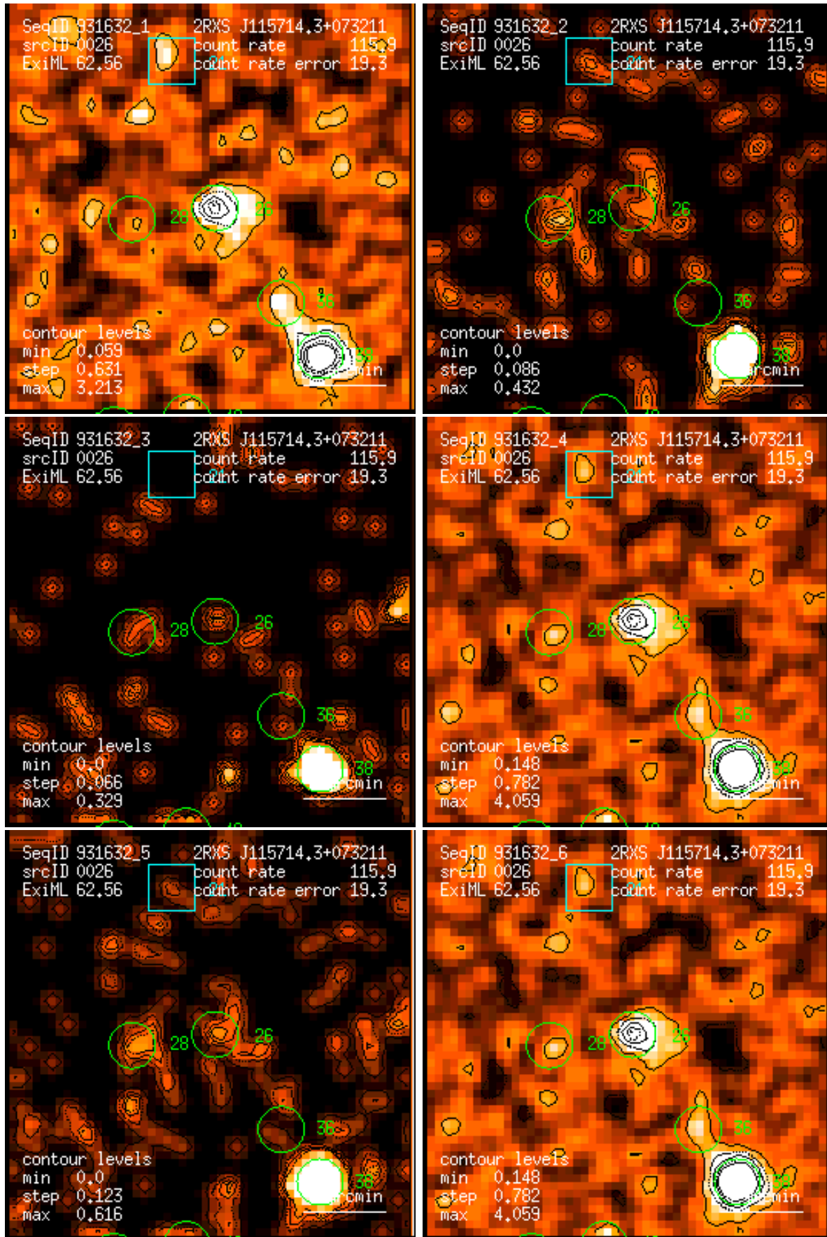
Figure 26: RASS 931632: detection 0026: band rate images, Gaussian filter: (1) PSPC channels 11 – 41, (2) 52 – 90, (3) 91 – 201, (4) 11 – 235, (5) 52 – 201, (6) 11 – 201. Broad band rates in counts/ks. Band rate contour levels in counts/ks/arcmin 2 .
