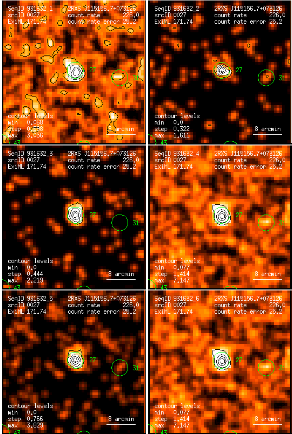
Figure 27: RASS 931632: detection 0027: band rate images, Gaussian filter: (1) PSPC channels 11 – 41, (2) 52 – 90, (3) 91 – 201, (4) 11 – 235, (5) 52 – 201, (6) 11 – 201. Broad band rates in counts/ks. Band rate contour levels in counts/ks/arcmin 2 .
