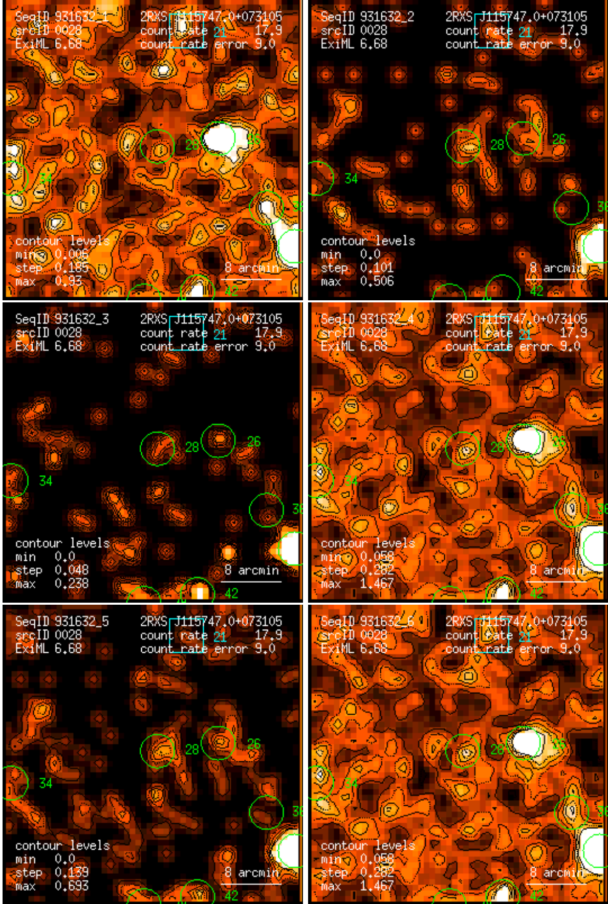
Figure 28: RASS 931632: detection 0028: band rate images, Gaussian filter: (1) PSPC channels 11 – 41, (2) 52 – 90, (3) 91 – 201, (4) 11 – 235, (5) 52 – 201, (6) 11 – 201. Broad band rates in counts/ks. Band rate contour levels in counts/ks/arcmin 2 .
