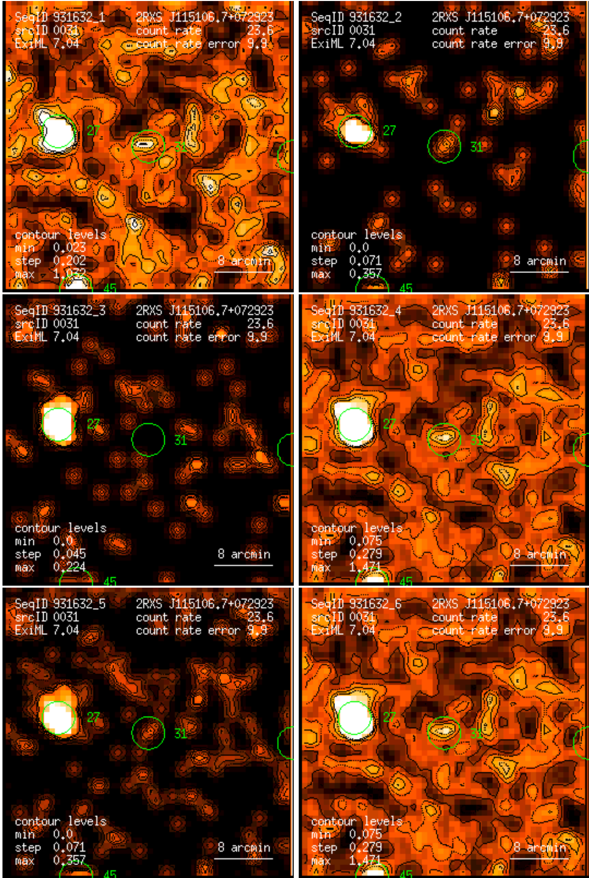
Figure 31: RASS 931632: detection 0031: band rate images, Gaussian filter: (1) PSPC channels 11 – 41, (2) 52 – 90, (3) 91 – 201, (4) 11 – 235, (5) 52 – 201, (6) 11 – 201. Broad band rates in counts/ks. Band rate contour levels in counts/ks/arcmin 2 .
