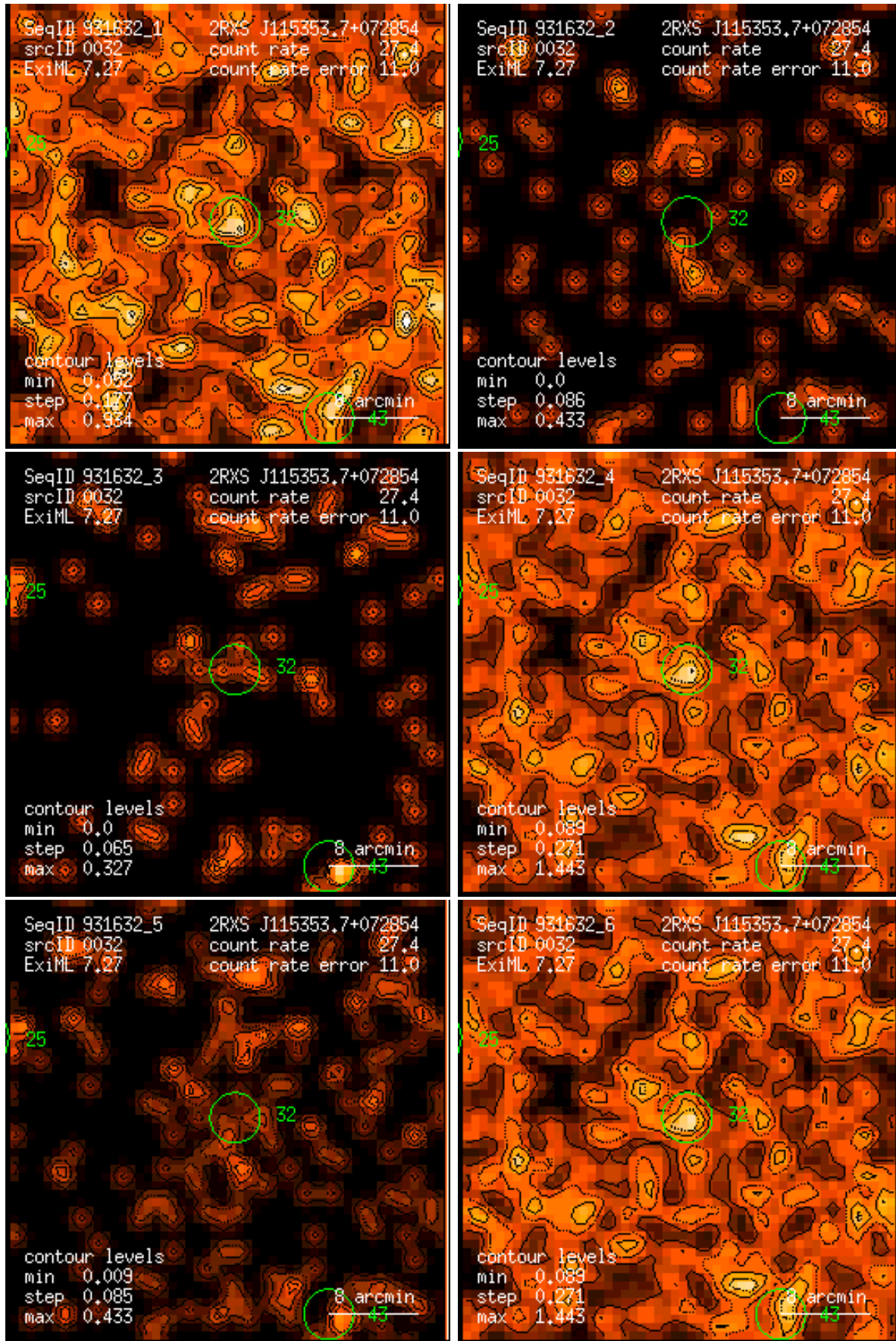
Figure 32: RASS 931632: detection 0032: band rate images, Gaussian filter: (1) PSPC channels 11 – 41, (2) 52 – 90, (3) 91 – 201, (4) 11 – 235, (5) 52 – 201, (6) 11 – 201. Broad band rates in counts/ks. Band rate contour levels in counts/ks/arcmin 2 .
