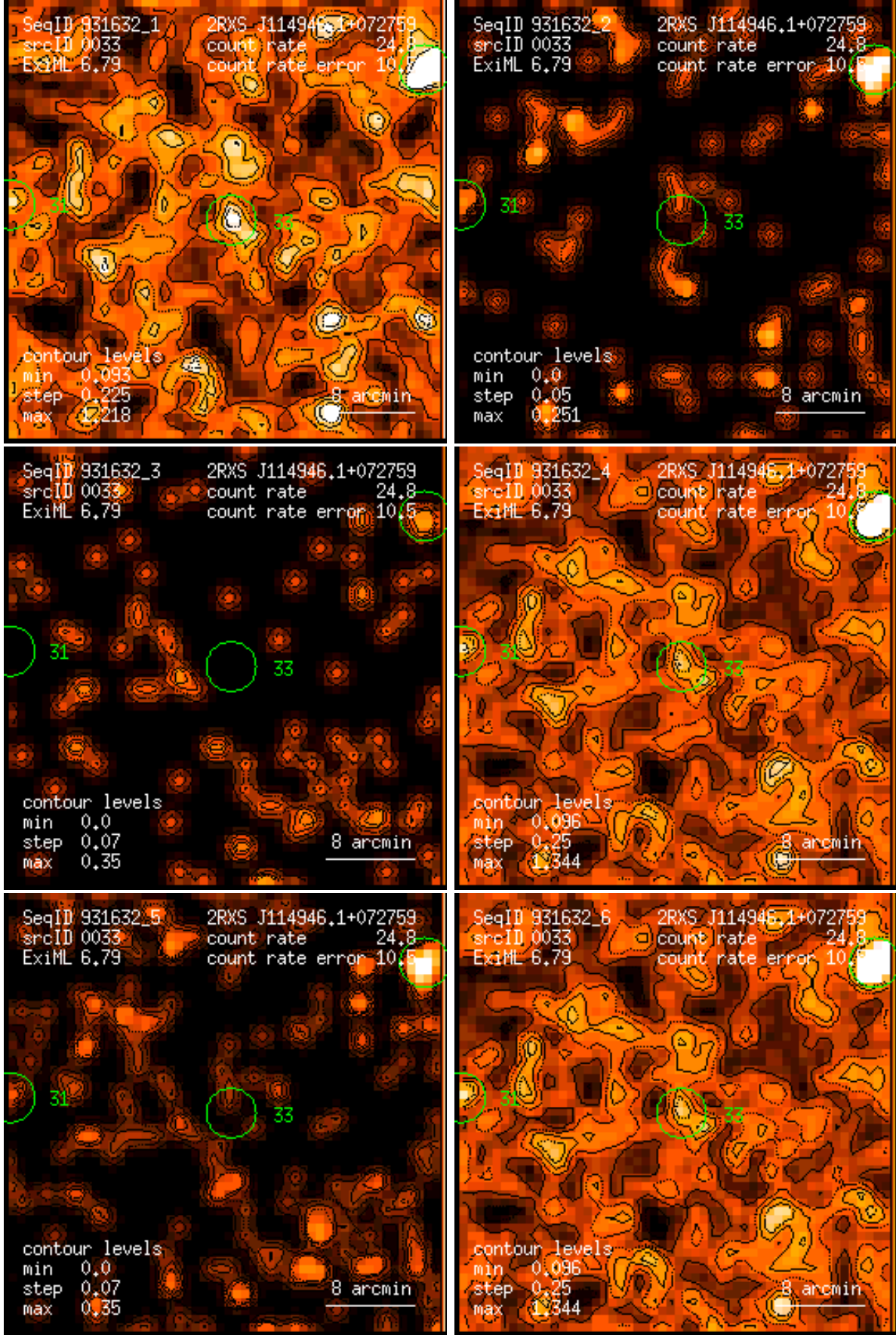
Figure 33: RASS 931632: detection 0033: band rate images, Gaussian filter: (1) PSPC channels 11 – 41, (2) 52 – 90, (3) 91 – 201, (4) 11 – 235, (5) 52 – 201, (6) 11 – 201. Broad band rates in counts/ks. Band rate contour levels in counts/ks/arcmin 2 .
