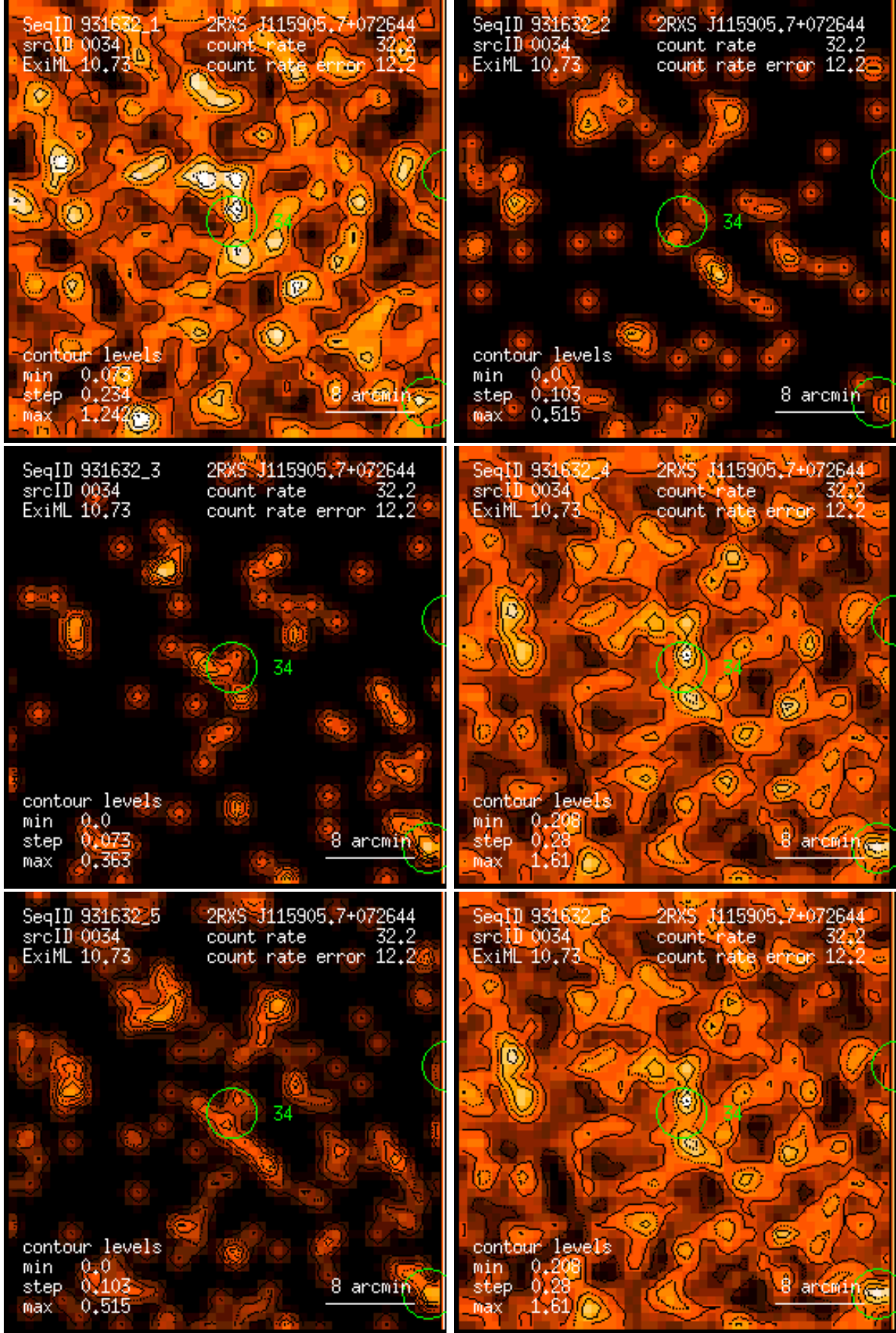
Figure 34: RASS 931632: detection 0034: band rate images, Gaussian filter: (1) PSPC channels 11 – 41, (2) 52 – 90, (3) 91 – 201, (4) 11 – 235, (5) 52 – 201, (6) 11 – 201. Broad band rates in counts/ks. Band rate contour levels in counts/ks/arcmin 2 .
