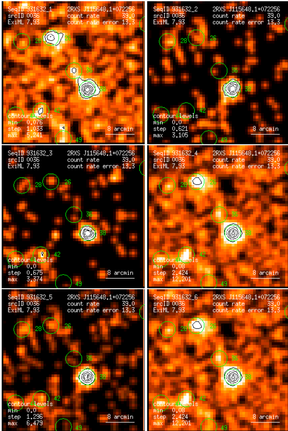
Figure 36: RASS 931632: detection 0036: band rate images, Gaussian filter: (1) PSPC channels 11 – 41, (2) 52 – 90, (3) 91 – 201, (4) 11 – 235, (5) 52 – 201, (6) 11 – 201. Broad band rates in counts/ks. Band rate contour levels in counts/ks/arcmin 2 .
