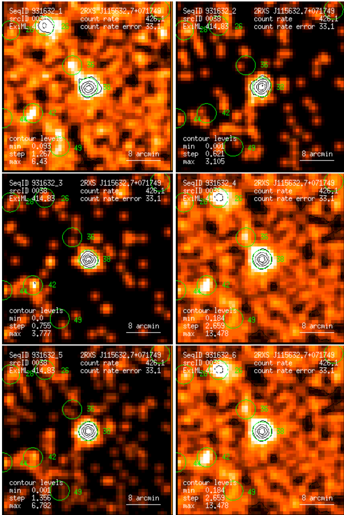
Figure 38: RASS 931632: detection 0038: band rate images, Gaussian filter: (1) PSPC channels 11 – 41, (2) 52 – 90, (3) 91 – 201, (4) 11 – 235, (5) 52 – 201, (6) 11 – 201. Broad band rates in counts/ks. Band rate contour levels in counts/ks/arcmin 2 .
