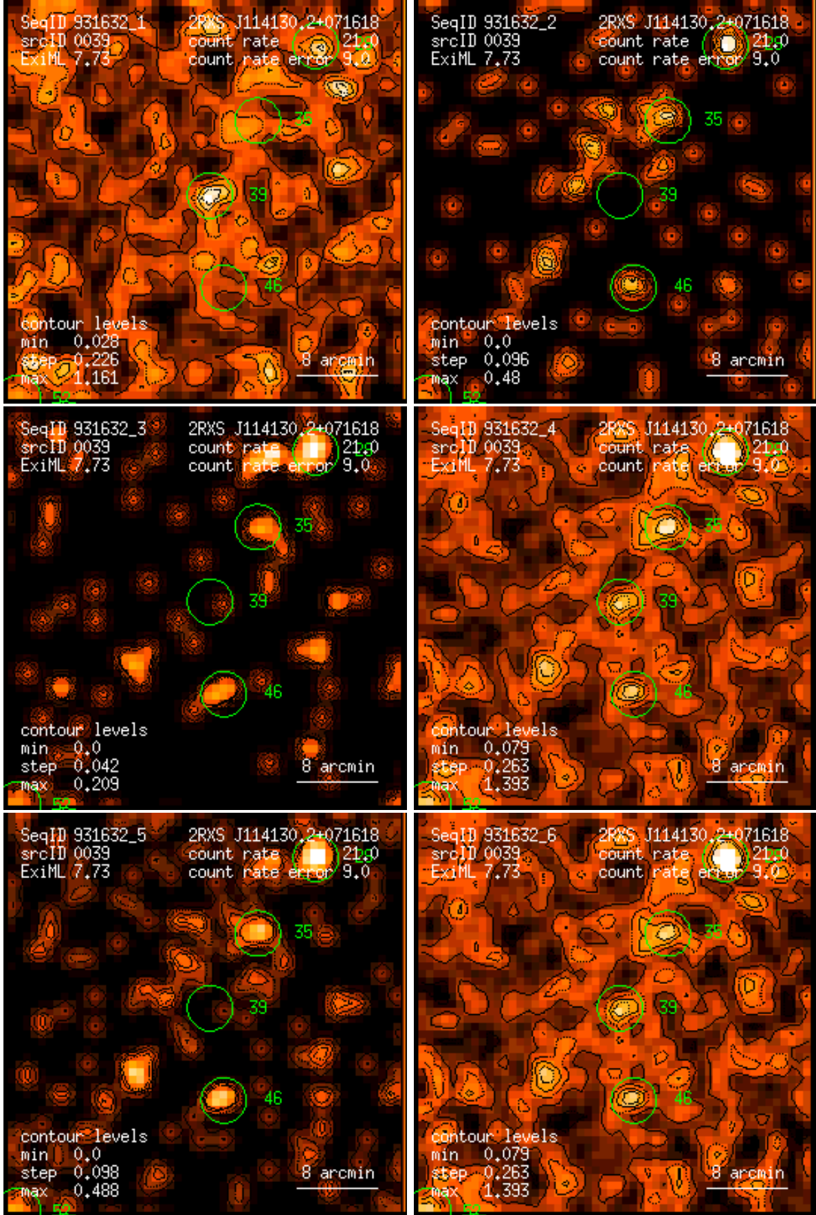
Figure 39: RASS 931632: detection 0039: band rate images, Gaussian filter: (1) PSPC channels 11 – 41, (2) 52 – 90, (3) 91 – 201, (4) 11 – 235, (5) 52 – 201, (6) 11 – 201. Broad band rates in counts/ks. Band rate contour levels in counts/ks/arcmin 2 .
