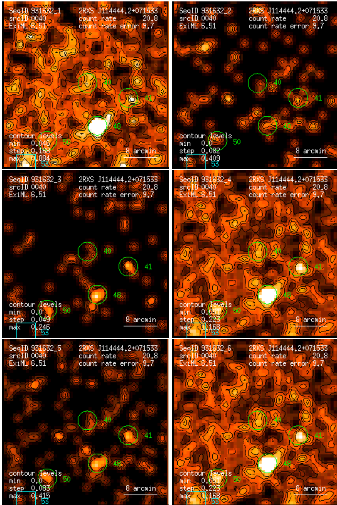
Figure 40: RASS 931632: detection 0040: band rate images, Gaussian filter: (1) PSPC channels 11 – 41, (2) 52 – 90, (3) 91 – 201, (4) 11 – 235, (5) 52 – 201, (6) 11 – 201. Broad band rates in counts/ks. Band rate contour levels in counts/ks/arcmin 2 .
