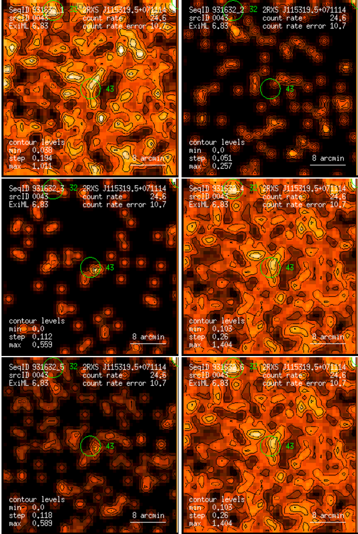
Figure 43: RASS 931632: detection 0043: band rate images, Gaussian filter: (1) PSPC channels 11 – 41, (2) 52 – 90, (3) 91 – 201, (4) 11 – 235, (5) 52 – 201, (6) 11 – 201. Broad band rates in counts/ks. Band rate contour levels in counts/ks/arcmin 2 .
