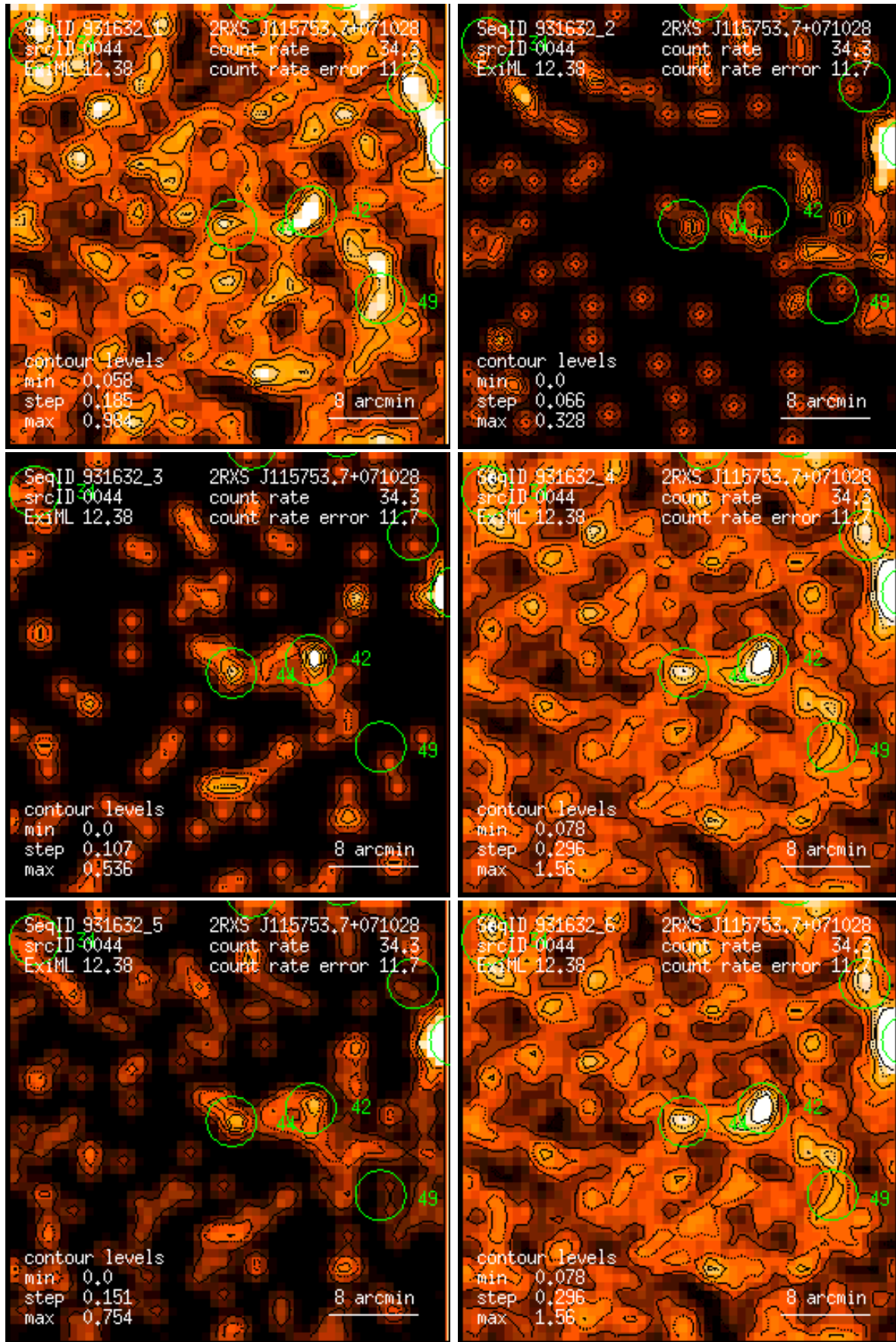
Figure 44: RASS 931632: detection 0044: band rate images, Gaussian filter: (1) PSPC channels 11 – 41, (2) 52 – 90, (3) 91 – 201, (4) 11 – 235, (5) 52 – 201, (6) 11 – 201. Broad band rates in counts/ks. Band rate contour levels in counts/ks/arcmin 2 .
