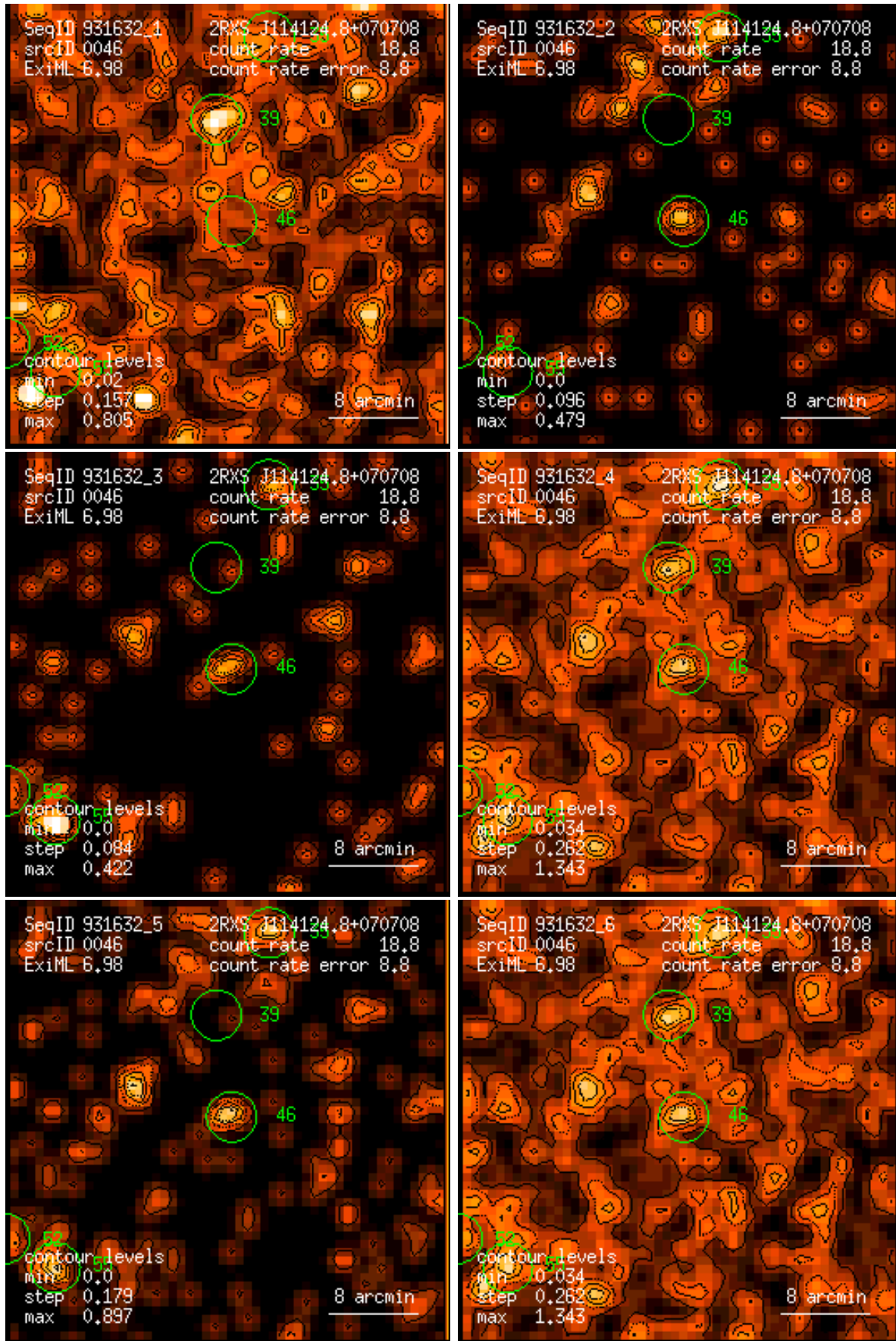
Figure 46: RASS 931632: detection 0046: band rate images, Gaussian filter: (1) PSPC channels 11 – 41, (2) 52 – 90, (3) 91 – 201, (4) 11 – 235, (5) 52 – 201, (6) 11 – 201. Broad band rates in counts/ks. Band rate contour levels in counts/ks/arcmin 2 .
