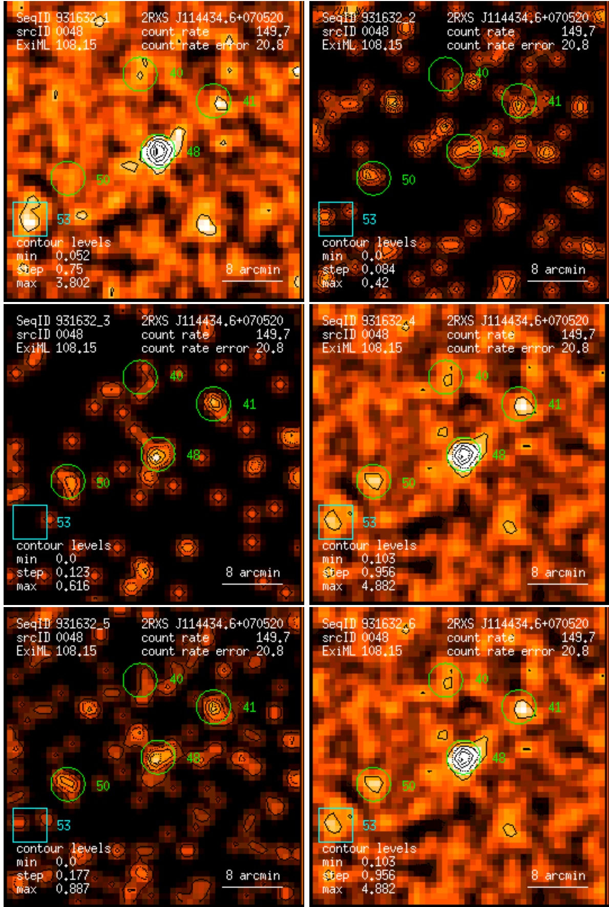
Figure 48: RASS 931632: detection 0048: band rate images, Gaussian filter: (1) PSPC channels 11 – 41, (2) 52 – 90, (3) 91 – 201, (4) 11 – 235, (5) 52 – 201, (6) 11 – 201. Broad band rates in counts/ks. Band rate contour levels in counts/ks/arcmin 2 .
