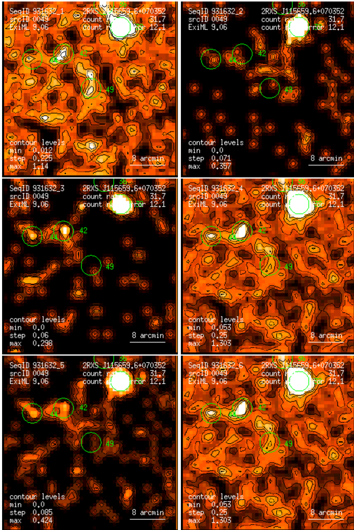
Figure 49: RASS 931632: detection 0049: band rate images, Gaussian filter: (1) PSPC channels 11 – 41, (2) 52 – 90, (3) 91 – 201, (4) 11 – 235, (5) 52 – 201, (6) 11 – 201. Broad band rates in counts/ks. Band rate contour levels in counts/ks/arcmin 2 .
