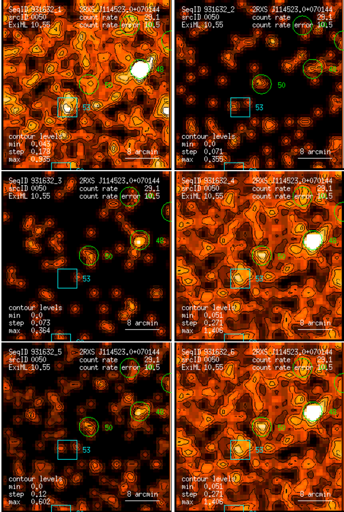
Figure 50: RASS 931632: detection 0050: band rate images, Gaussian filter: (1) PSPC channels 11 – 41, (2) 52 – 90, (3) 91 – 201, (4) 11 – 235, (5) 52 – 201, (6) 11 – 201. Broad band rates in counts/ks. Band rate contour levels in counts/ks/arcmin 2 .
