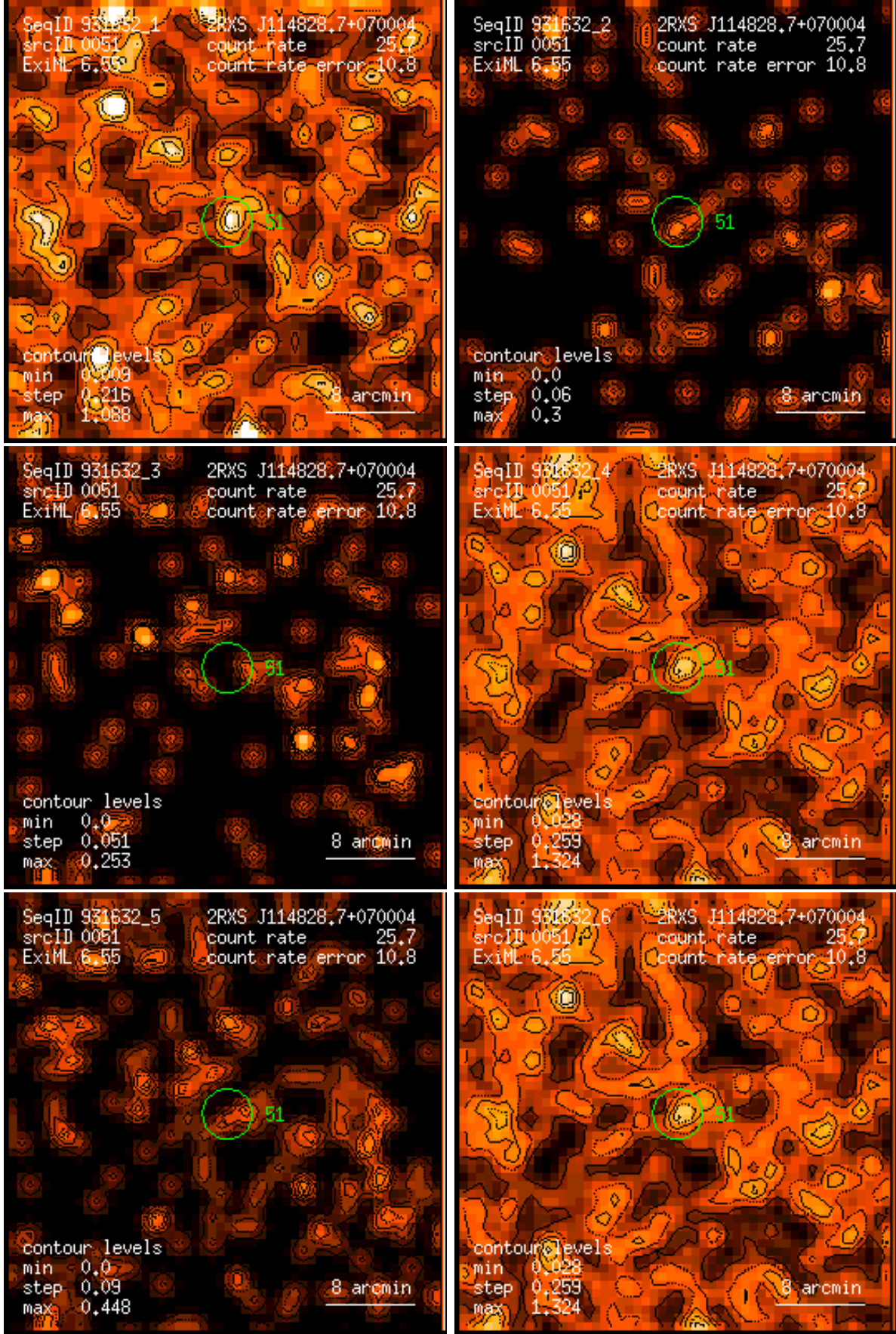
Figure 51: RASS 931632: detection 0051: band rate images, Gaussian filter: (1) PSPC channels 11 – 41, (2) 52 – 90, (3) 91 – 201, (4) 11 – 235, (5) 52 – 201, (6) 11 – 201. Broad band rates in counts/ks. Band rate contour levels in counts/ks/arcmin 2 .
