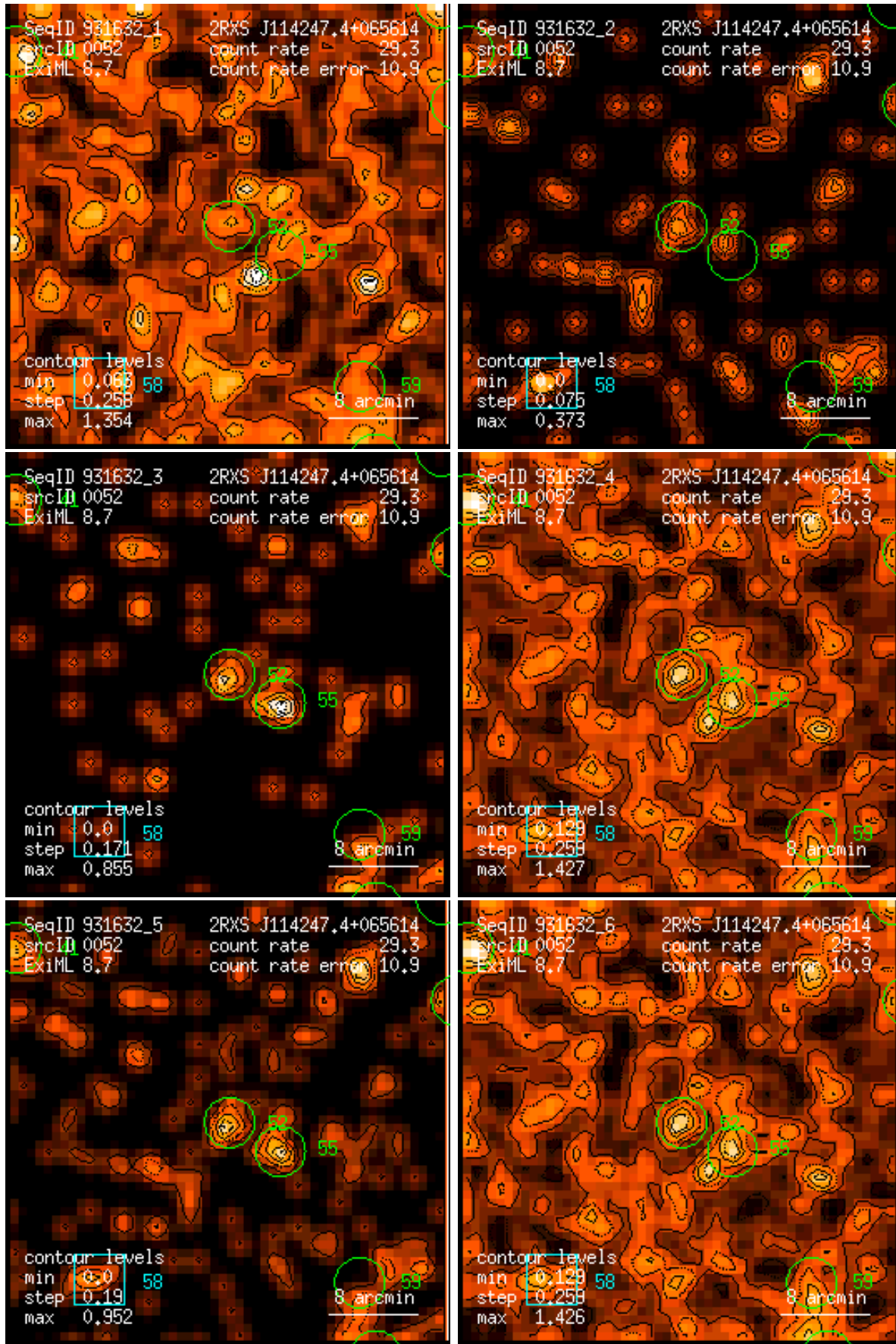
Figure 52: RASS 931632: detection 0052: band rate images, Gaussian filter: (1) PSPC channels 11 – 41, (2) 52 – 90, (3) 91 – 201, (4) 11 – 235, (5) 52 – 201, (6) 11 – 201. Broad band rates in counts/ks. Band rate contour levels in counts/ks/arcmin 2 .
