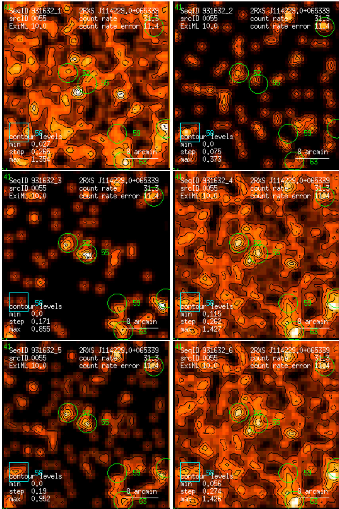
Figure 55: RASS 931632: detection 0055: band rate images, Gaussian filter: (1) PSPC channels 11 – 41, (2) 52 – 90, (3) 91 – 201, (4) 11 – 235, (5) 52 – 201, (6) 11 – 201. Broad band rates in counts/ks. Band rate contour levels in counts/ks/arcmin 2 .
